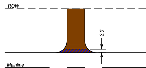
(15) Field Entrance D 3' from Edge of Mainline Match Existing Entrance Width
