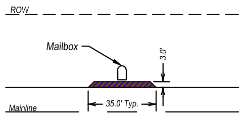
(15) Mailbox Pullout C 3' from Edge of Mainline
