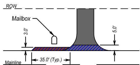
(15) Driveway Entrance with Mailbox A 3' / 5' from Edge of Mainline Match Existing Entrance Width
