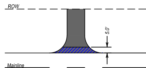
(15) Driveway Entrance B 5' from Edge of Mainline Match Existing Entrance Width
