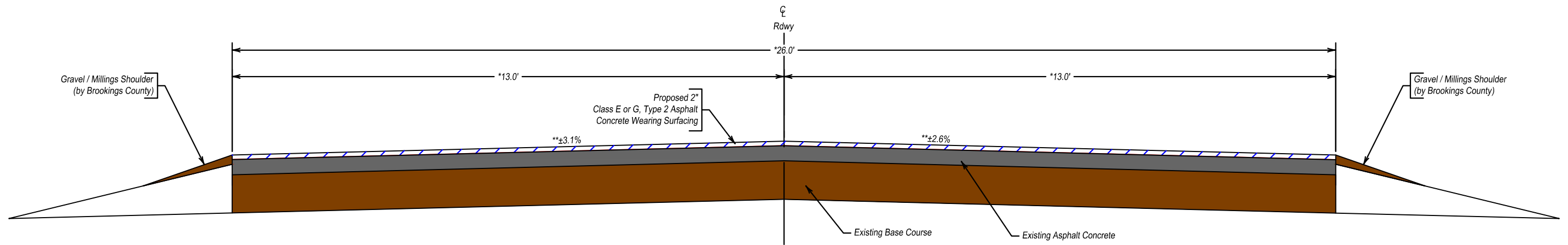
TYPICAL SURFACING SECTION Brookings County 25
